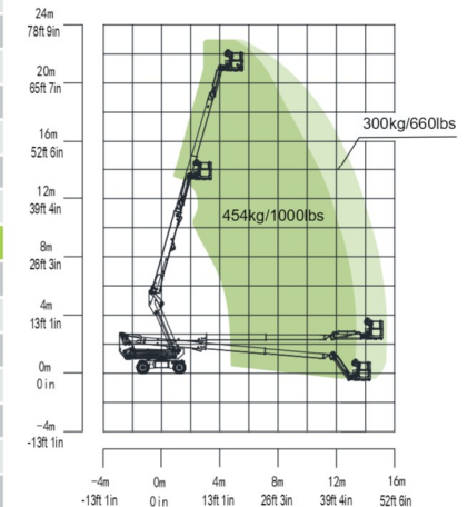
Range of Motion ZT21JEH-V
